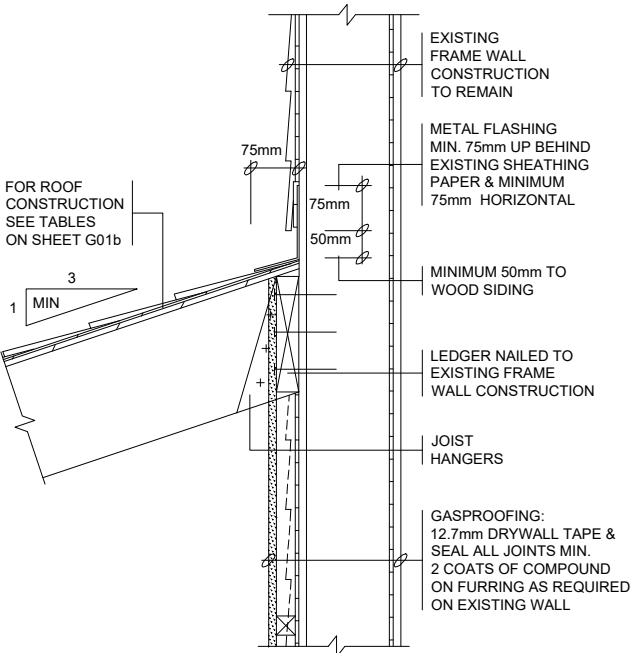
1 FRAME WALL
