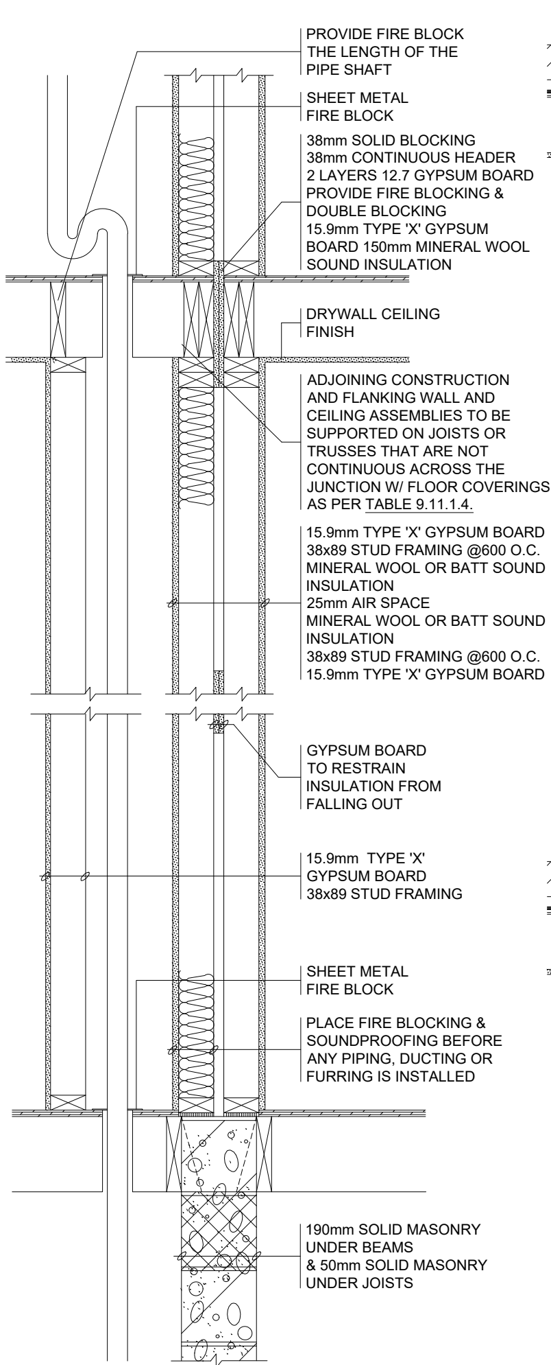
VERTICAL SECTION
