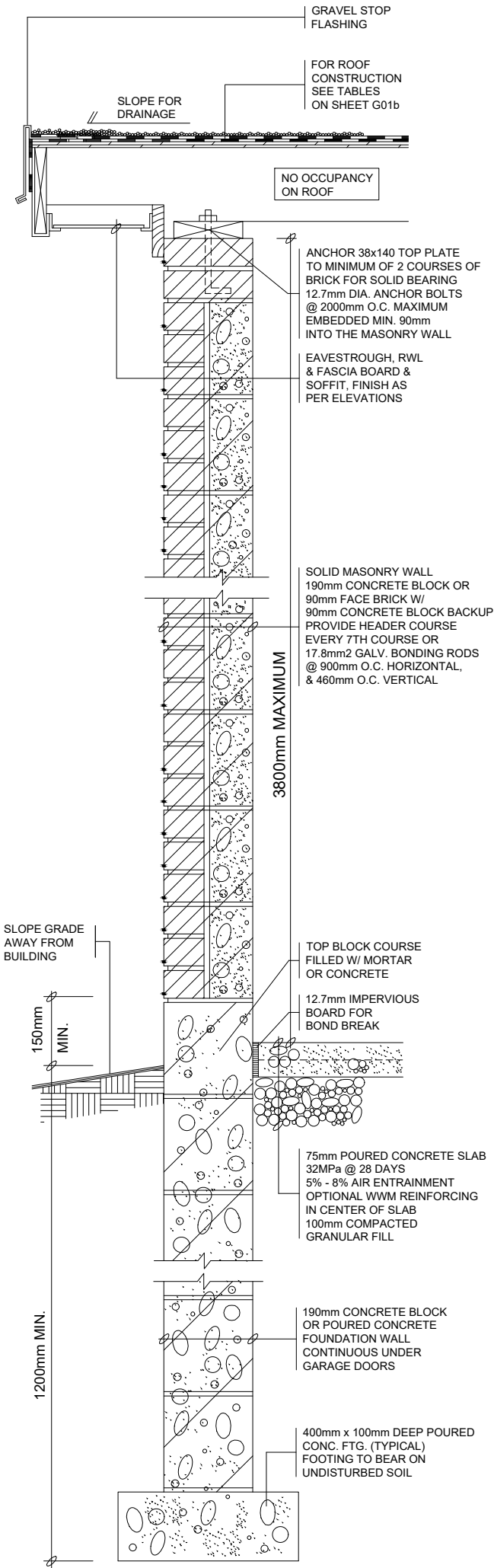
4 WALL SECTION
