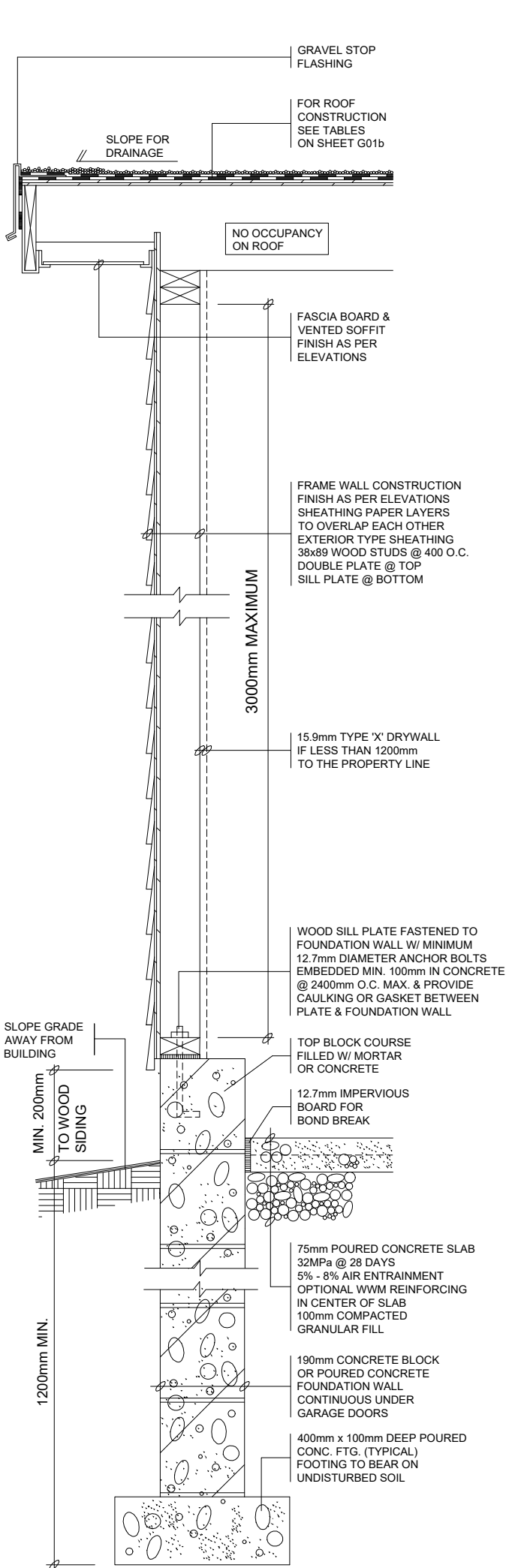
4 WALL SECTION
