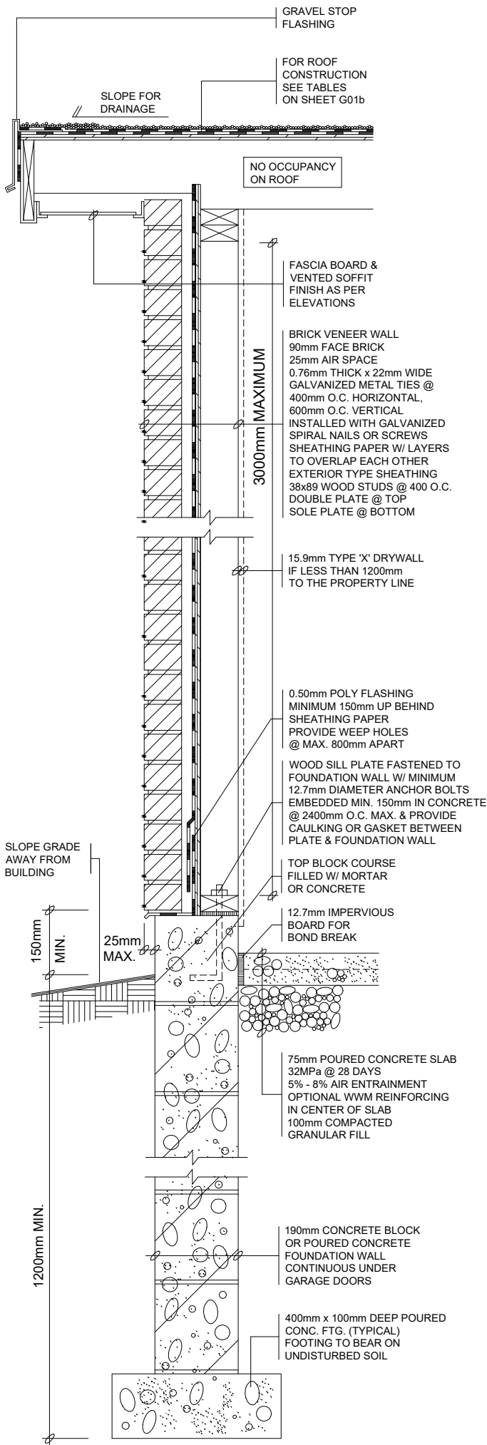
4 WALL SECTION
